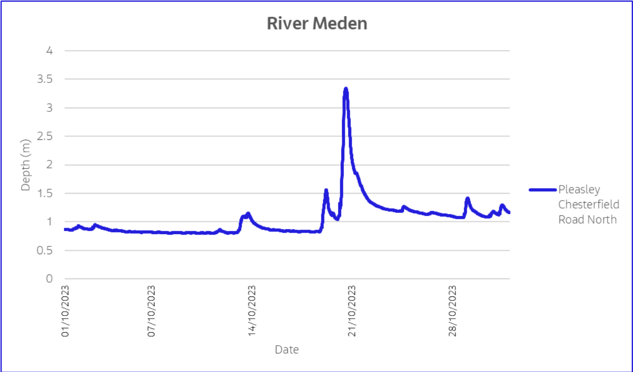
Figure 4-9: 15-minute river level data recorded in October 2023 from Pleasley Chesterfield Road North gauging station on the River Meden
