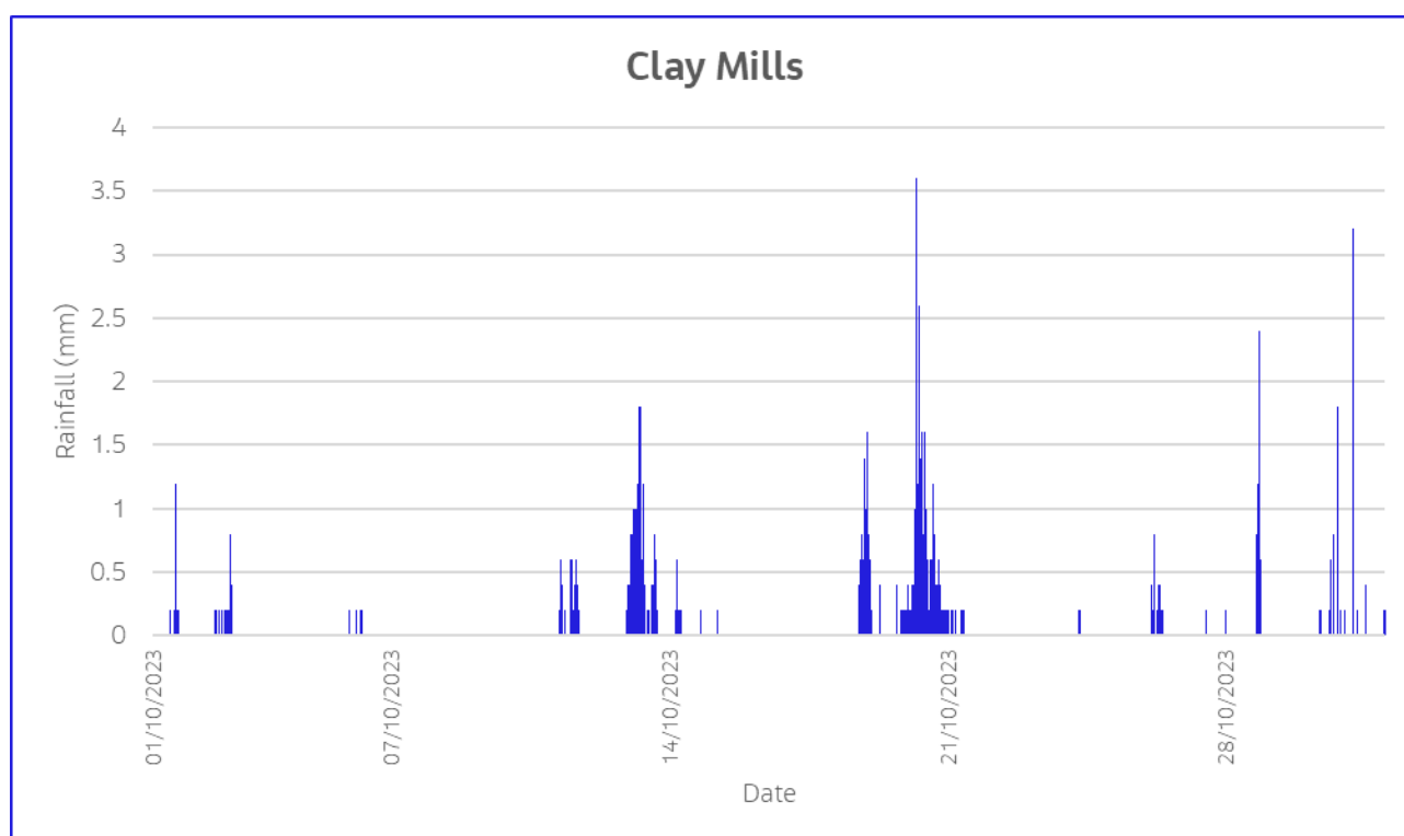
Figure 5-10: 15-minute rainfall data recorded in October 2023 at Clay Mills rain gauge
