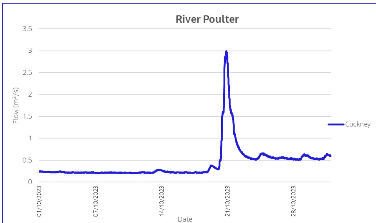
Figure 4-7: 15-minute river flow data recorded in October 2023 from Cuckney gauging station on the River Poulter
