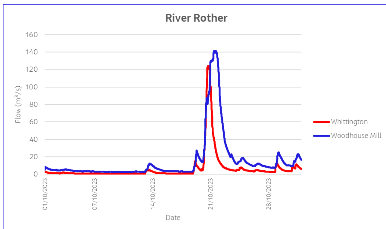
Figure 2-9: 15-minute river flow data recorded in October 2023 from Whittington and Woodhouse Mill gauging stations on the River Rother
