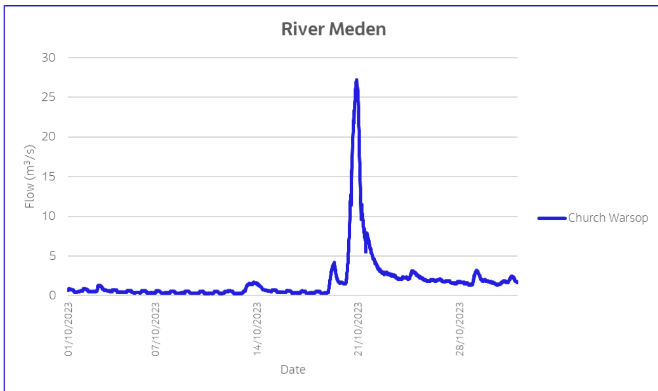
Figure 4-8: 15-minute river flow data recorded in October 2023 from Church Warsop gauging station on the River Meden
