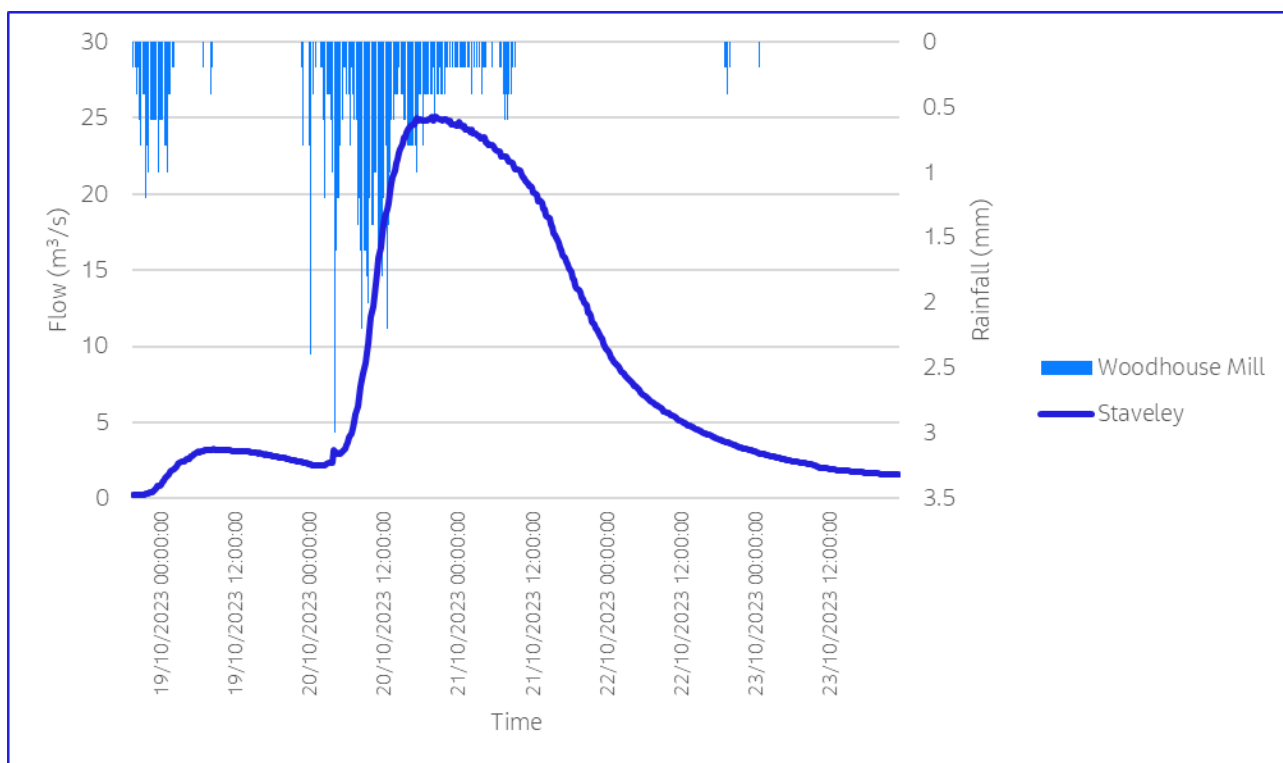
Figure 2-16: Hydrograph from the 19th to the 23rd of October illustrating recorded river flow data from Staveley gauging station and recorded rainfall data from Woodhouse Mill rain gauge
