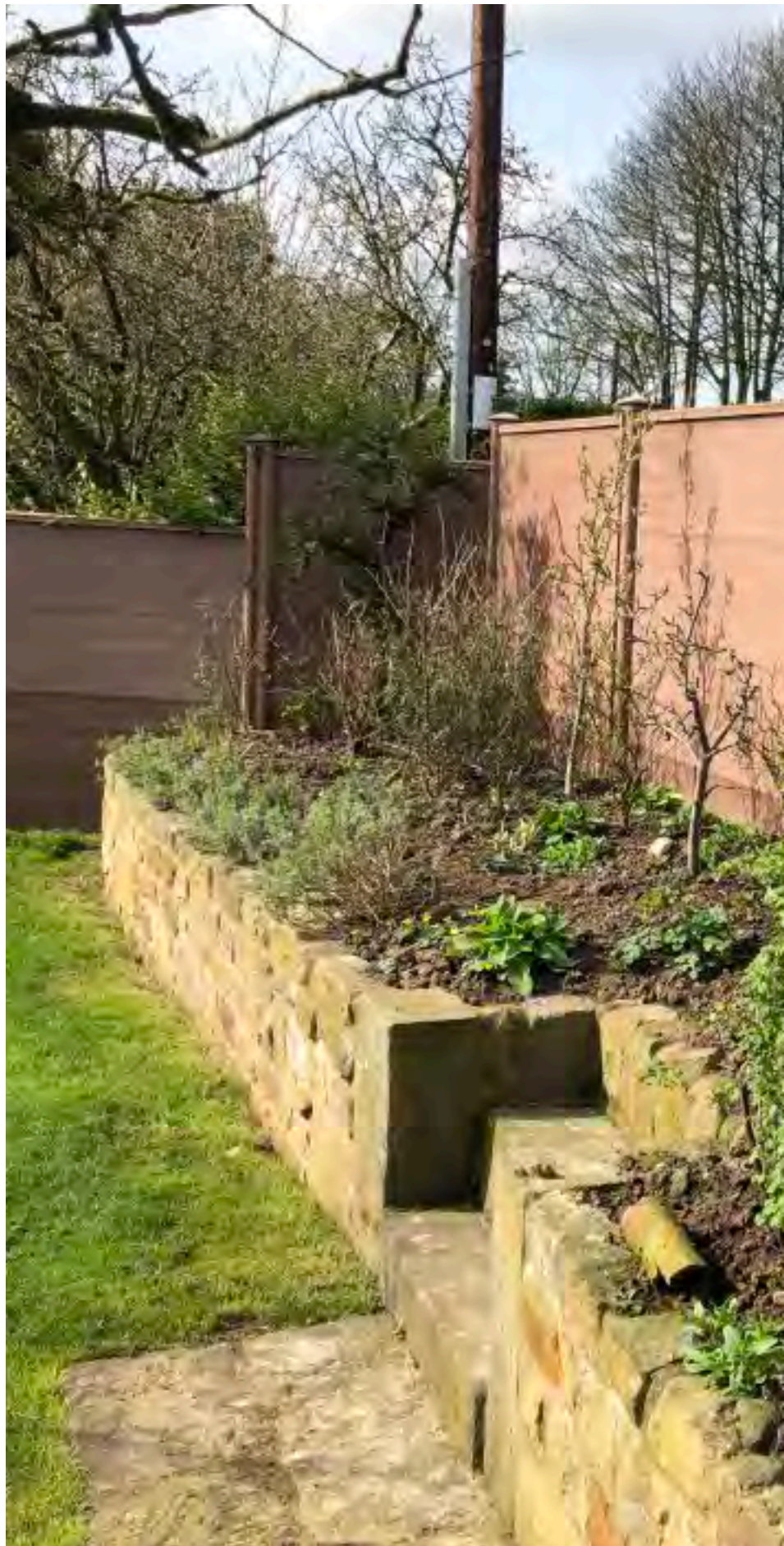
At the perimeter of the garden one-metre-deep holes were filled with concrete, into which posts and reinforced 'Task Green' waterproof fence panels were fitted.
